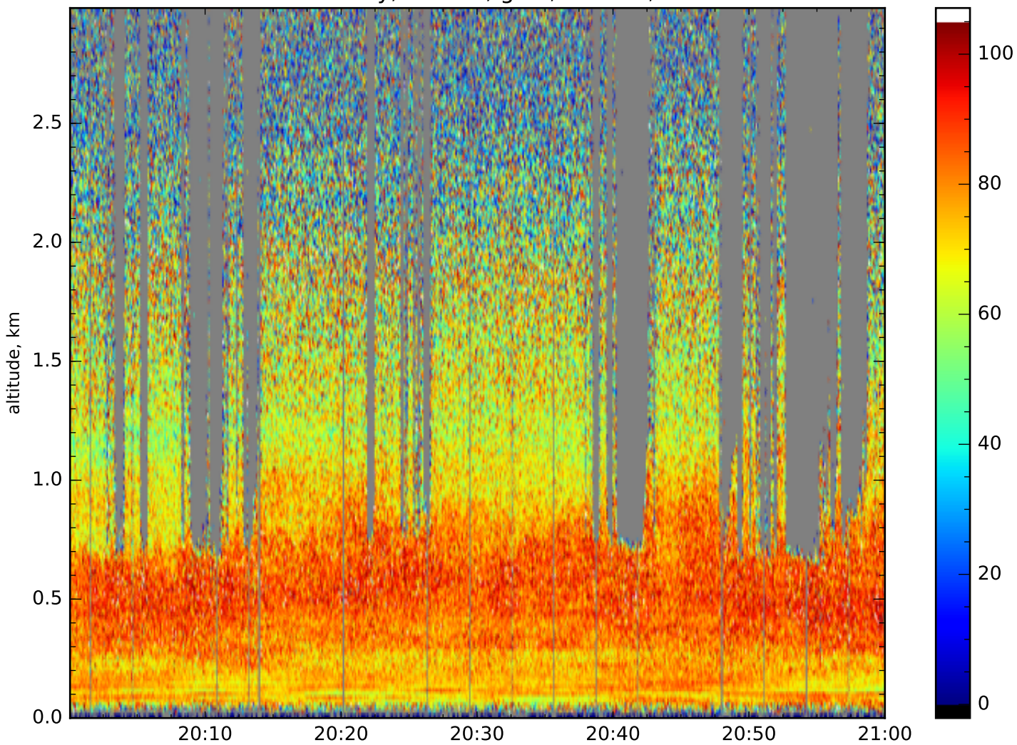
Relative humidity error, 355nm, glue, res.: 4s, 15-330m
