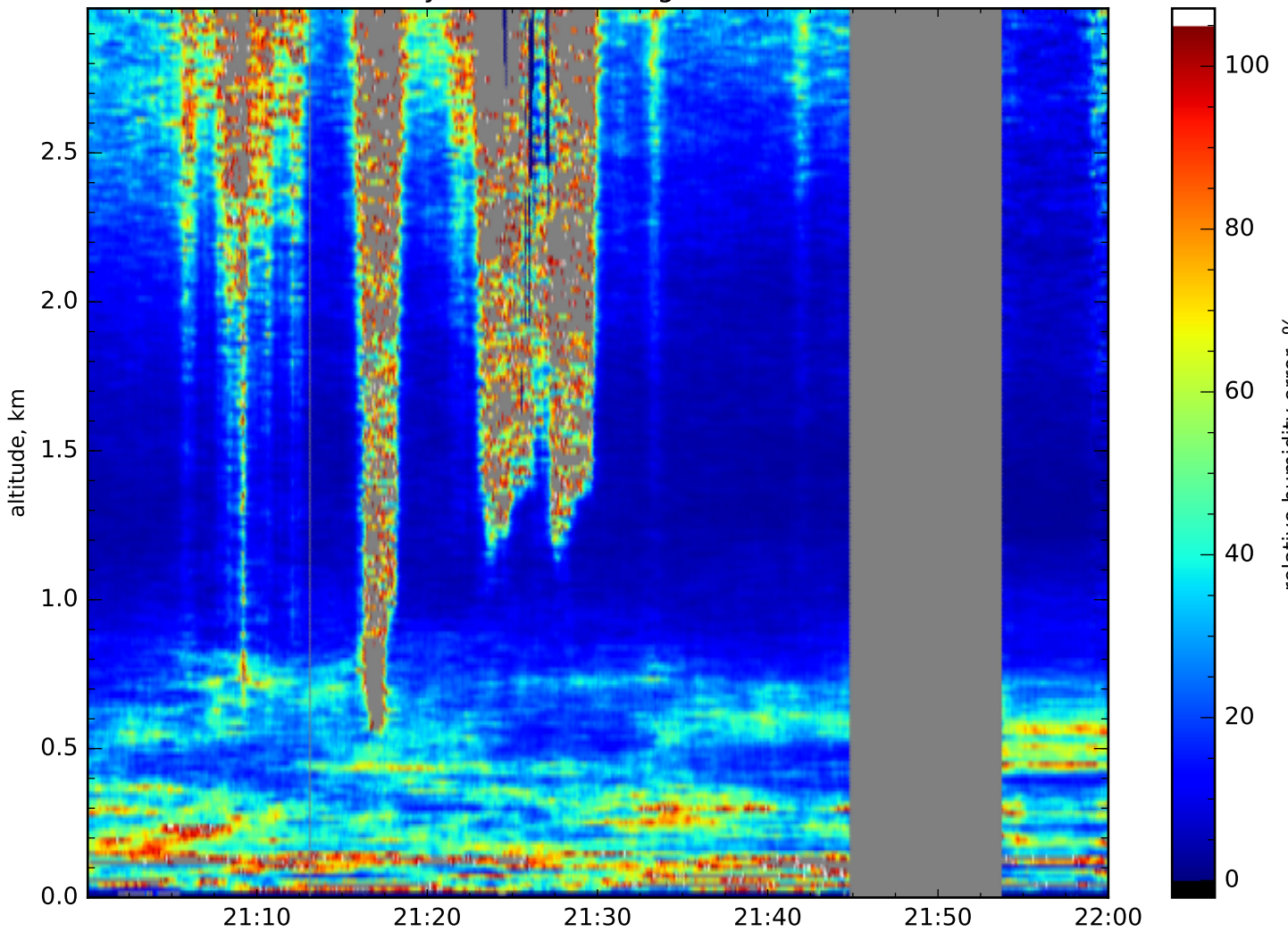
Relative humidity error, 355nm, glue, res.: 60s, 15-330m
