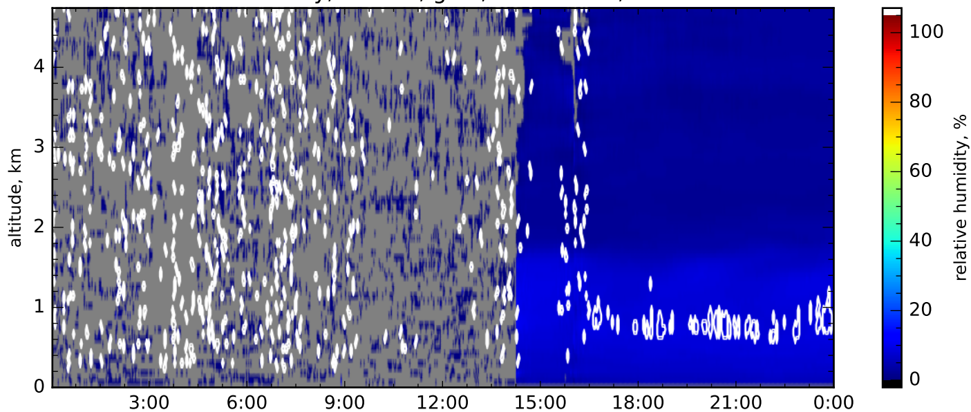
Relative humidity, 355nm, glue, res.: 3600s, 60m-420m
