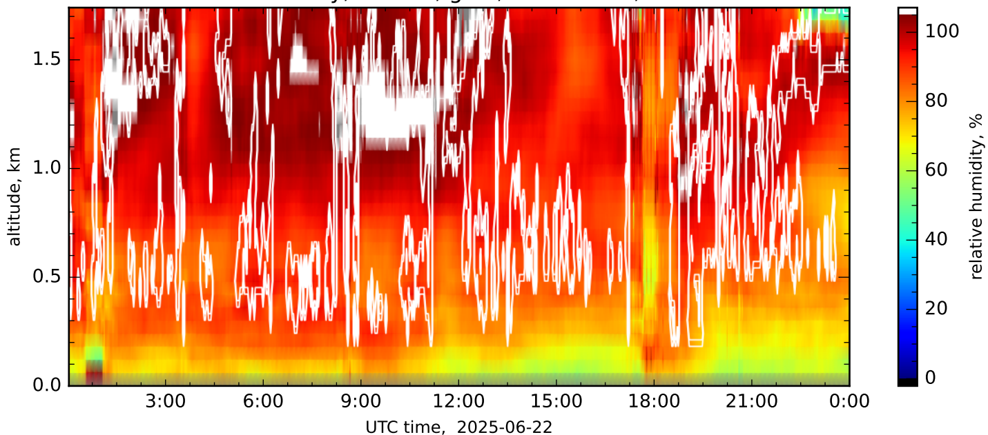
Relative humidity, 355nm, glue, res.: 3600s, 60m-180m
