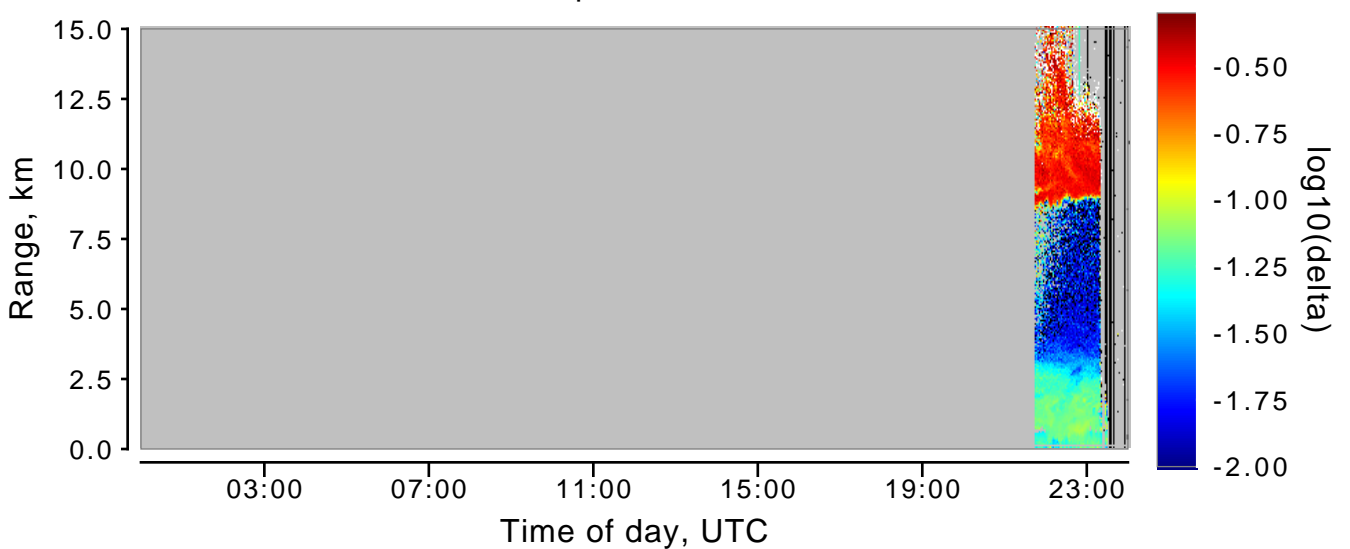
532nm volume depolarization ratio
