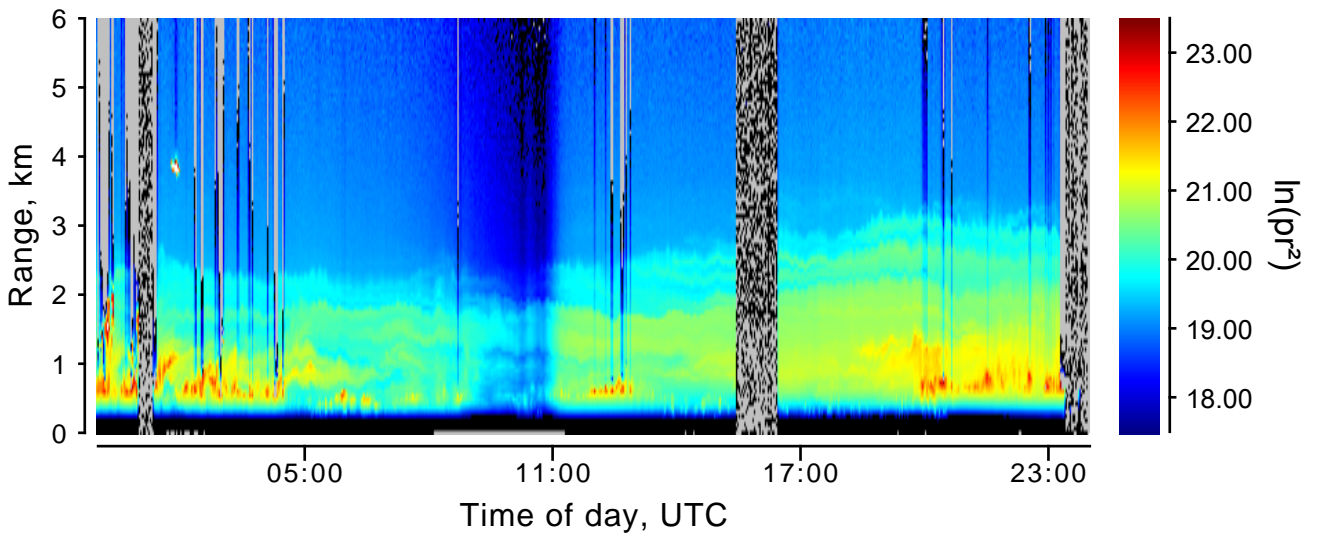
1064nm attenuated backscatter near range
