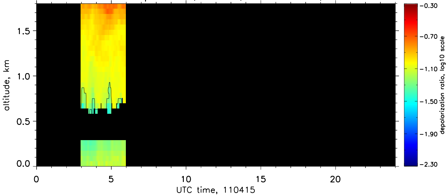
Particle linear depol. ratio, 532nm, res.: 10 min., 60–60 m
