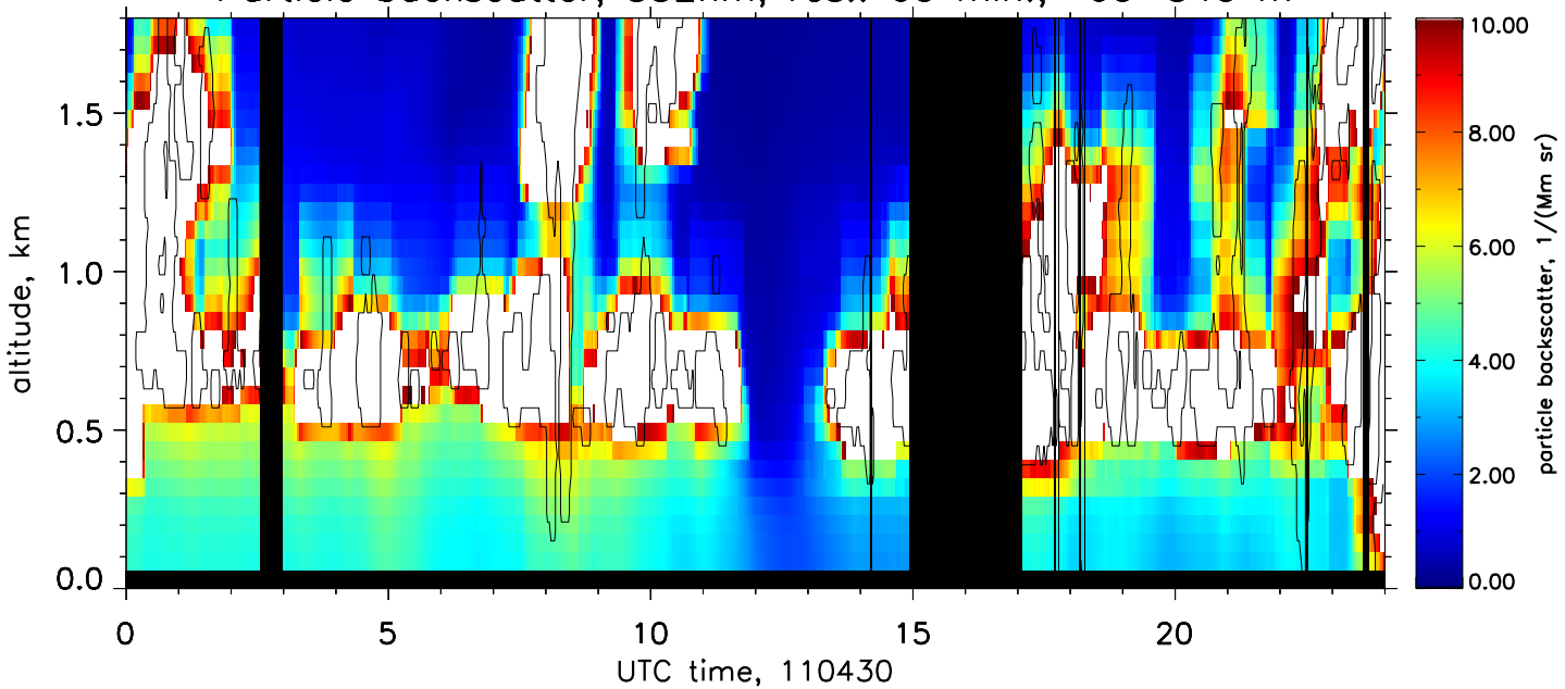
Particle backscatter, 532nm, res.: 60 min., 60–540 m
