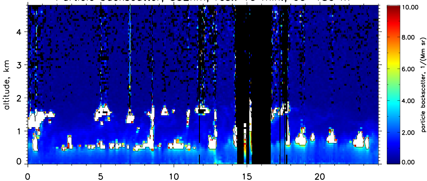
Particle backscatter, 532nm, res.: 10 min., 60–180 m
