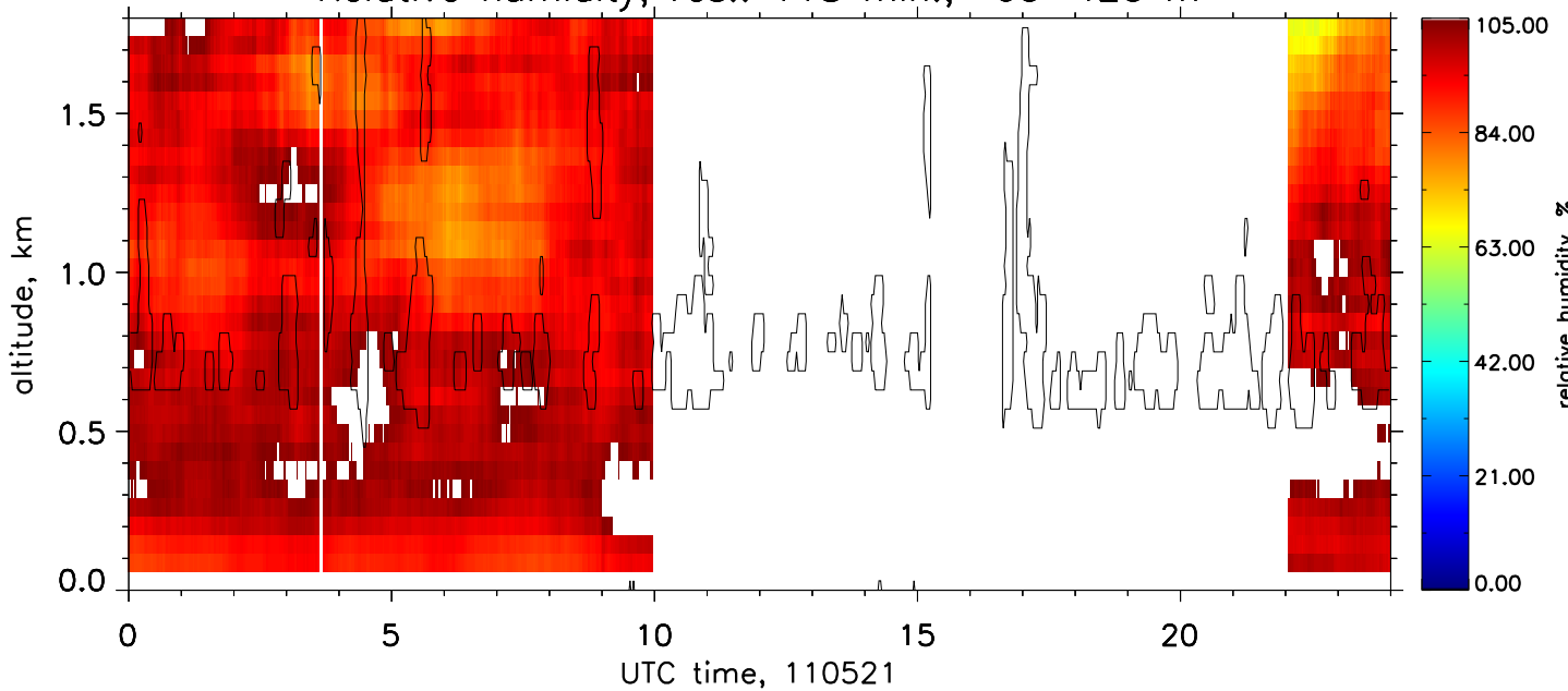
Relative humidity, res.: 118 min., 60–420 m
