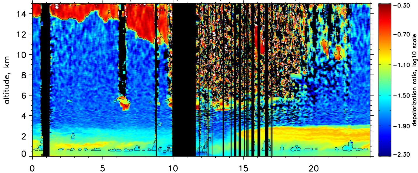
Volume linear depol. ratio, 532nm, res.: 10 min., 60–660 m
