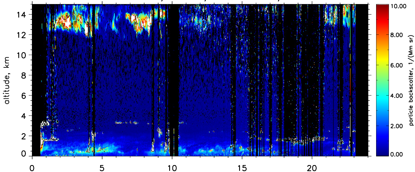
Particle backscatter, 532nm, res.: 2 min., 60–660 m
