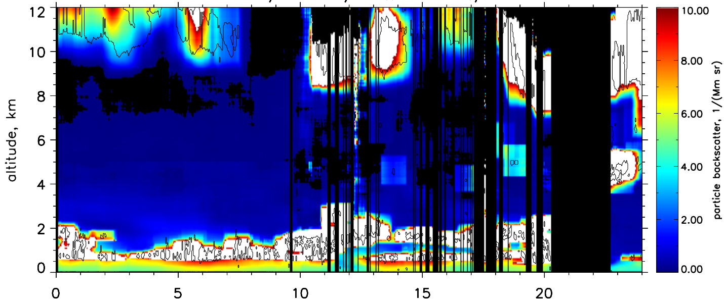
Particle backscatter, 355nm, res.: 60 min., 180–3300 m
