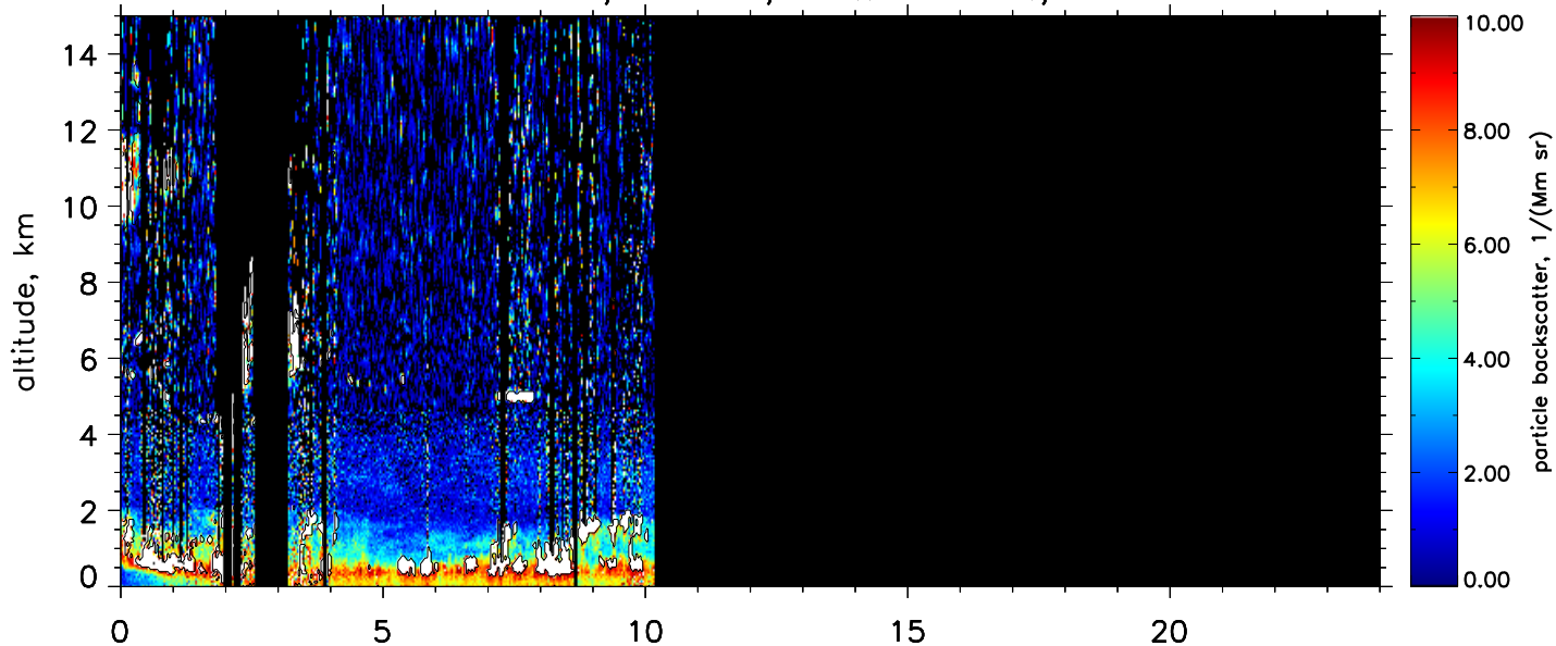
Particle backscatter, 355nm, res.: 2 min., 60–660 m
