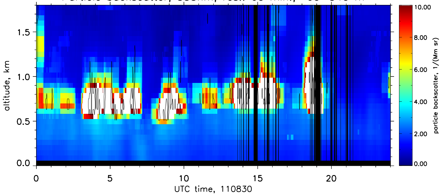
Particle backscatter, 355nm, res.: 60 min., 60–540 m
