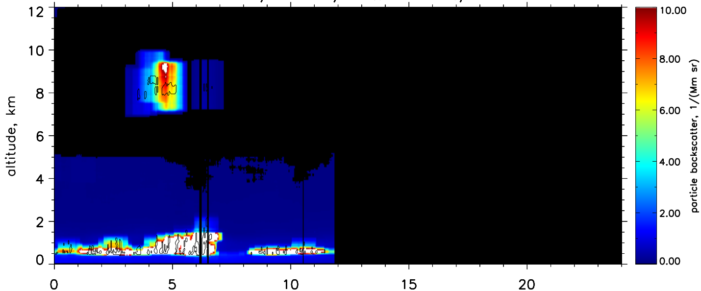
Particle backscatter, 532nm, res.: 60 min., 180–3300 m
