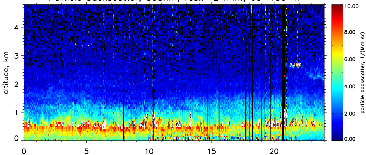
Particle backscatter, 355nm, res.: 2 min., 60–180 m
