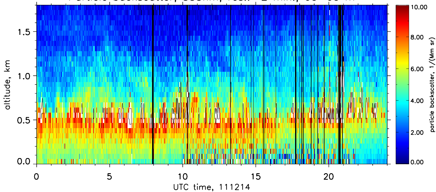
Particle backscatter, 355nm, res.: 2 min., 60–60 m
