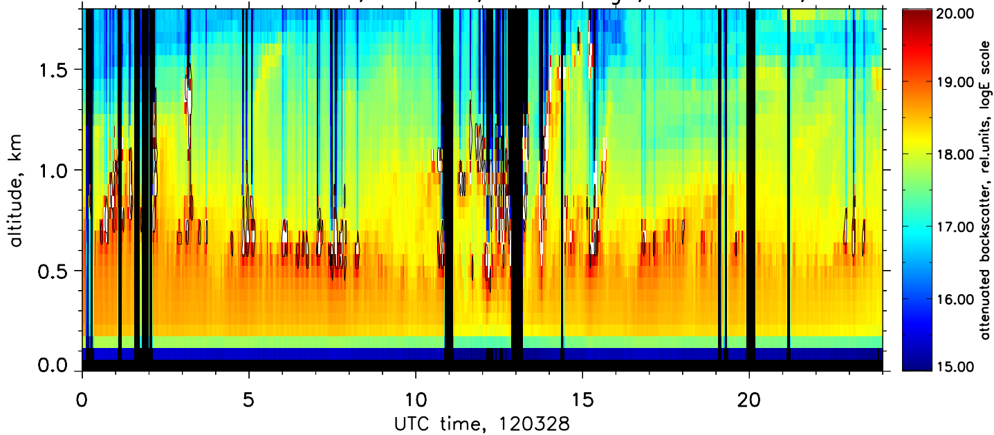
Attenuated backscatter, 1064nm, close range, res.: 2 min., 60 m
