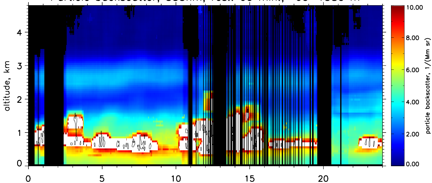
Particle backscatter, 355nm, res.: 60 min., 60–1380 m
