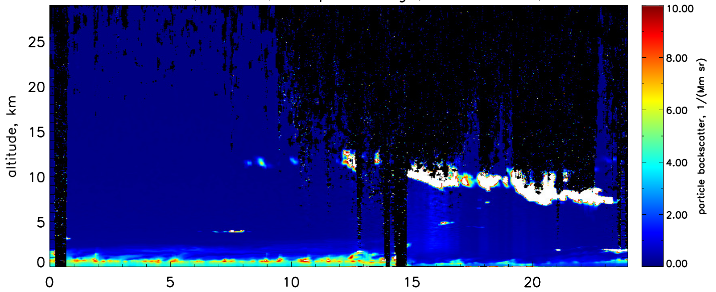
Particle backscatter, 532nm, complete range, res.: 10min., 60m–1.2km
