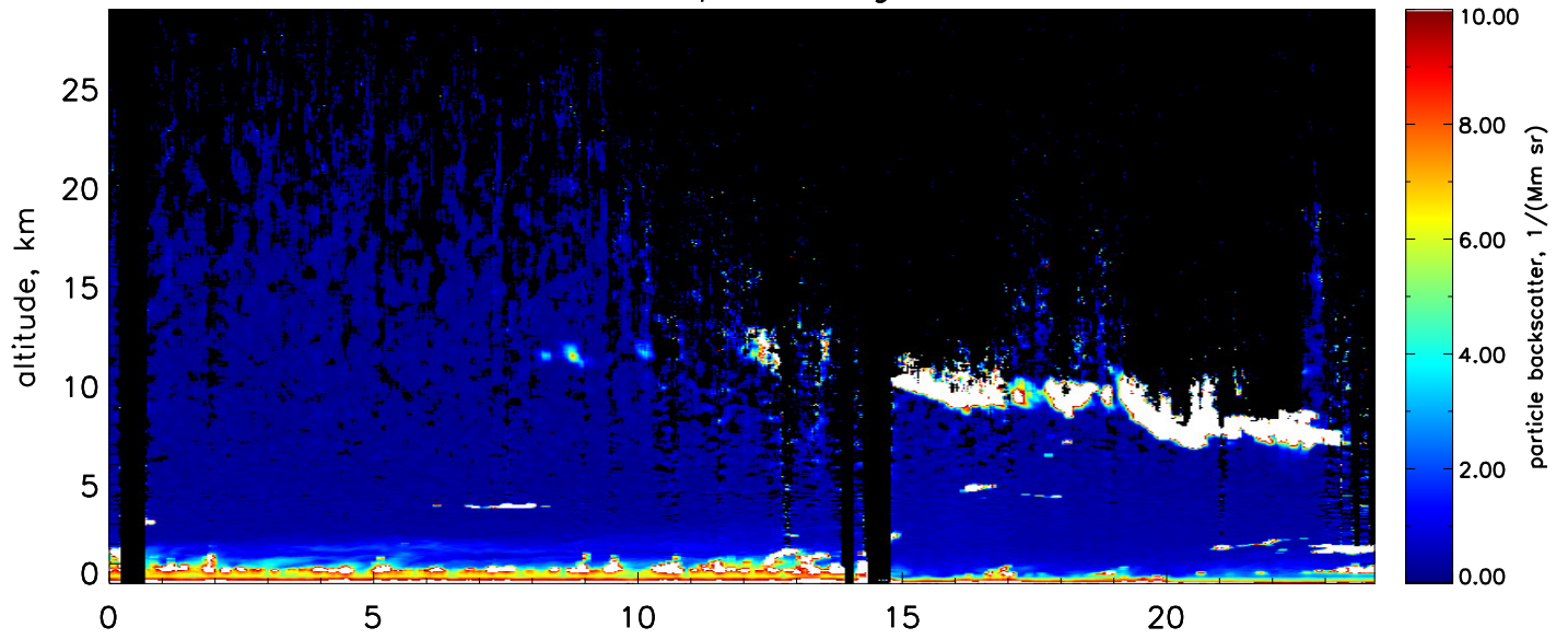
Particle backscatter, 355nm, complete range, res.: 10min., 60m–1.2km
