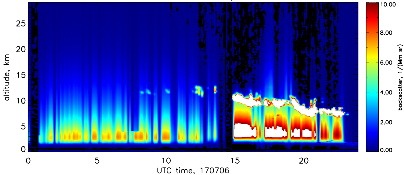
Attenuated backscatter, 355nm, 2nd telescope, res.: 10min., 60m–1.2km
