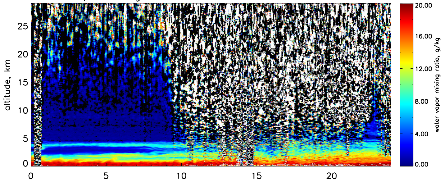
Water vapor mixing ratio, FAR+NEAR, res.: 10min., 60m-1.2km
