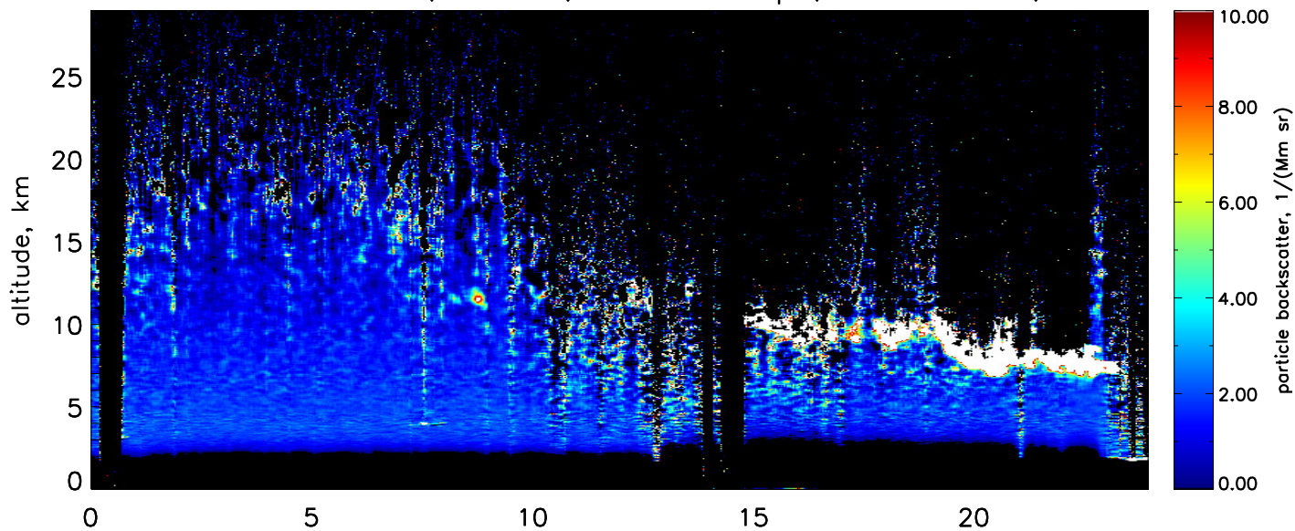
Particle backscatter, 355nm, 2nd telescope, res.: 10min., 60m
