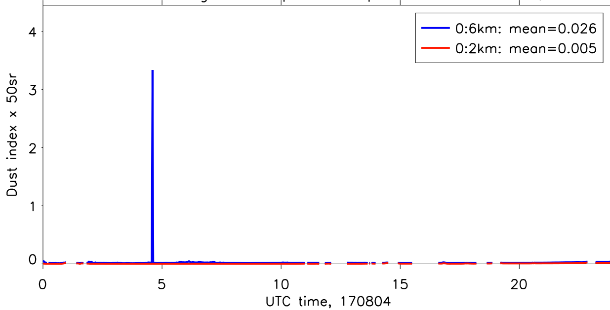
"Dust index": integrated depolarized particle backscatter, 532nm
