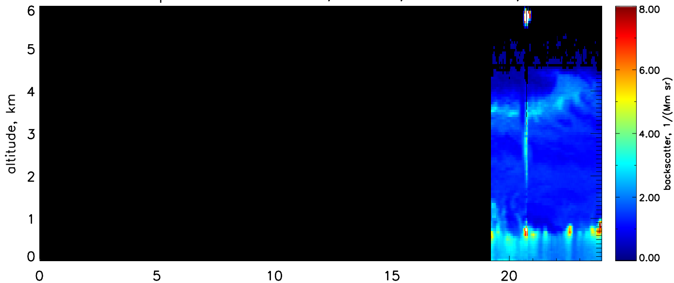
Polarized particle backscatter, 532nm, res.: 10min., 60m
