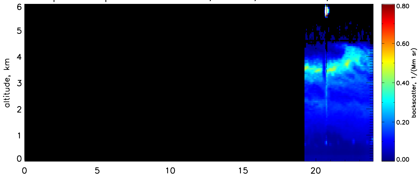
Depolarized particle backscatter, 532nm, res.: 10min., 60m
