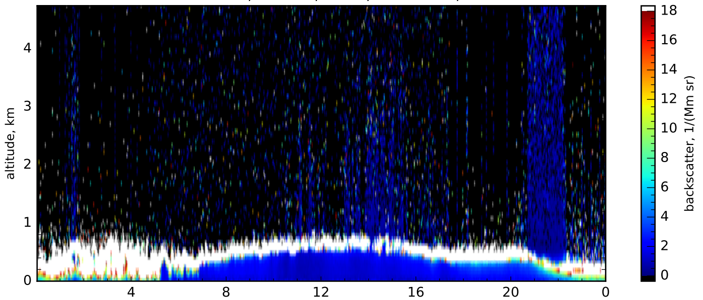
Particle backscatter, 532nm, close, res.: 120s, 60m-180m
