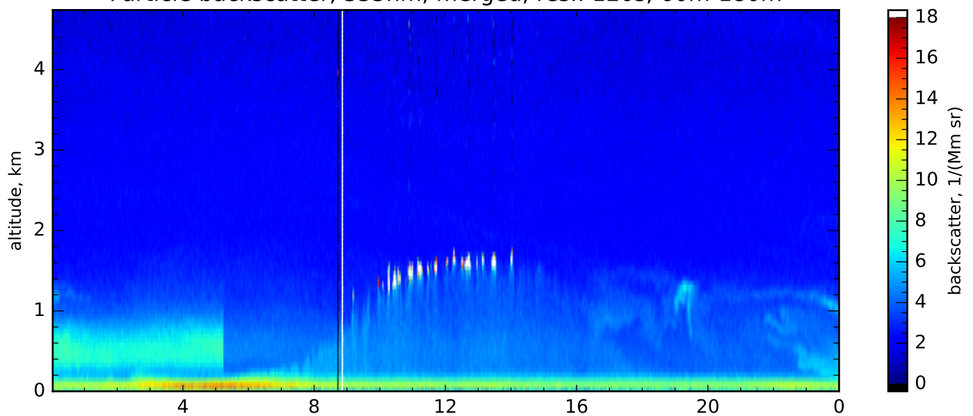
Particle backscatter, 355nm, merged, res.: 120s, 60m-180m
