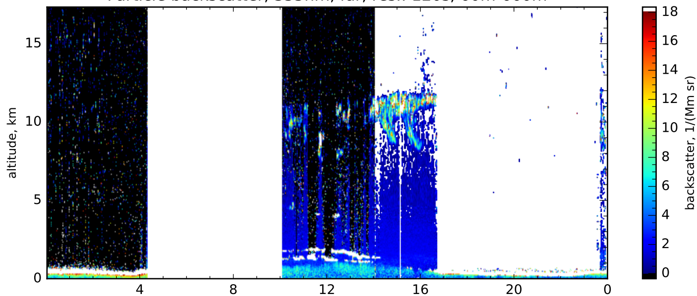
Particle backscatter, 355nm, far, res.: 120s, 60m-660m
