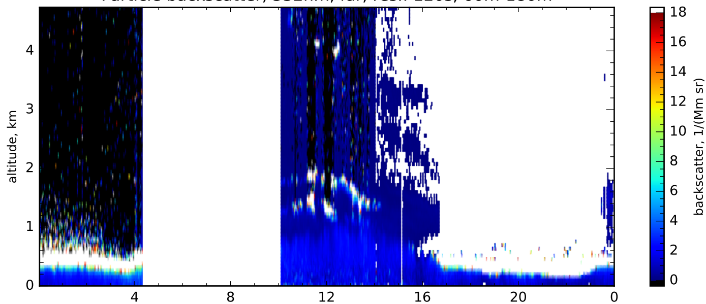
Particle backscatter, 532nm, far, res.: 120s, 60m-180m
