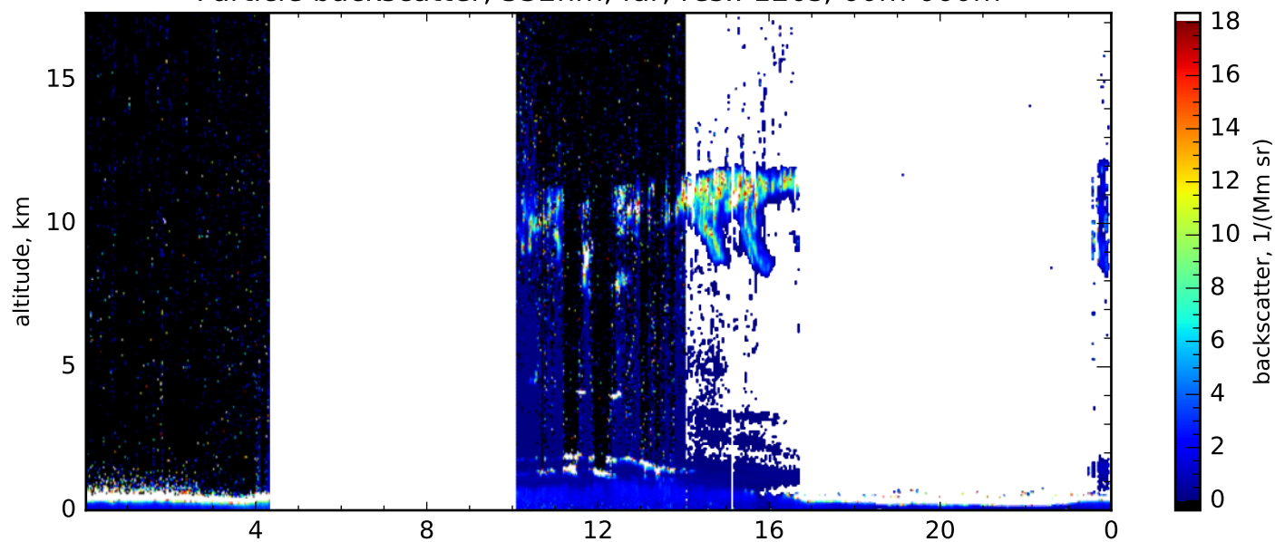
Particle backscatter, 532nm, far, res.: 120s, 60m-660m
