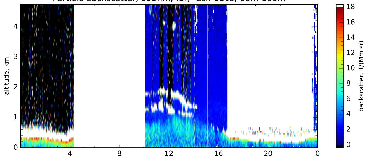
Particle backscatter, 355nm, far, res.: 120s, 60m-180m
