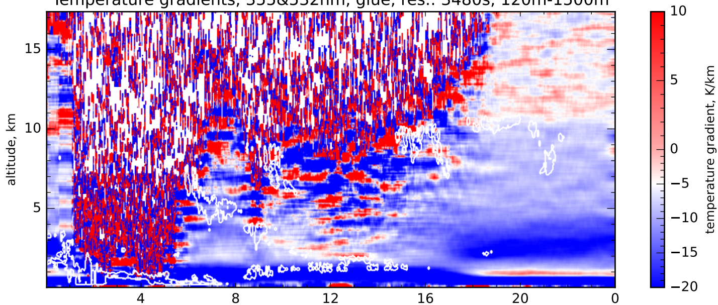
Temperature gradients, 355&532nm, glue, res.: 3480s, 120m-1500m
