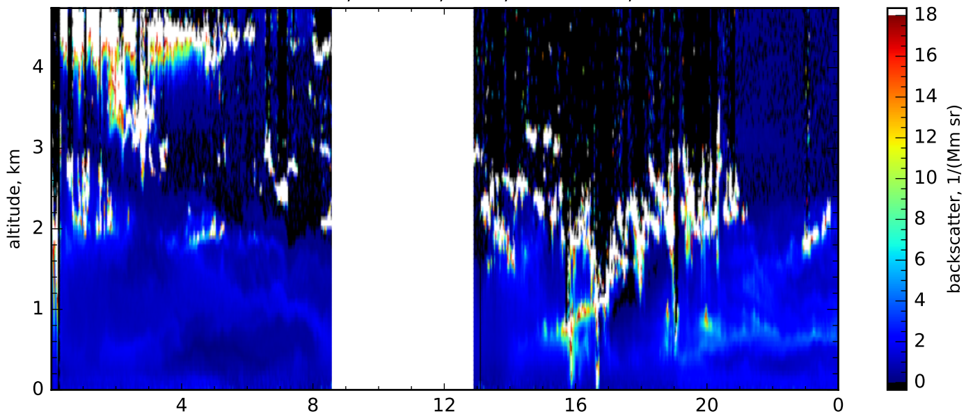
Particle backscatter, 532nm, near, res.: 120s, 60m-180m
