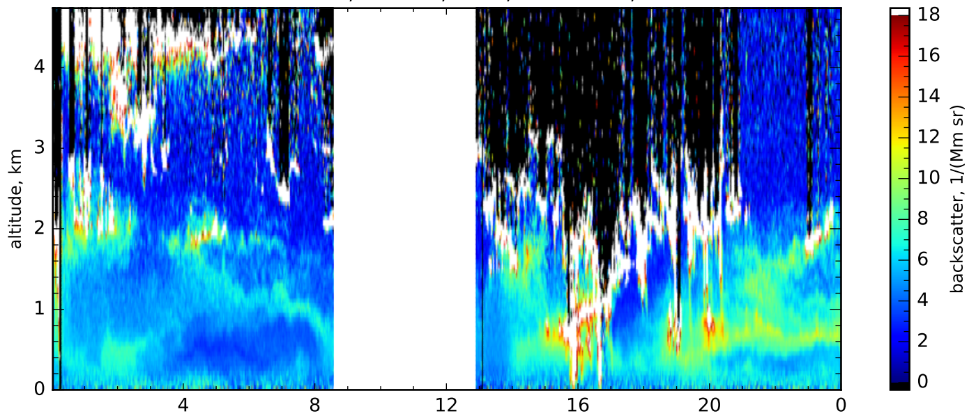
Particle backscatter, 355nm, near, res.: 120s, 60m-180m
