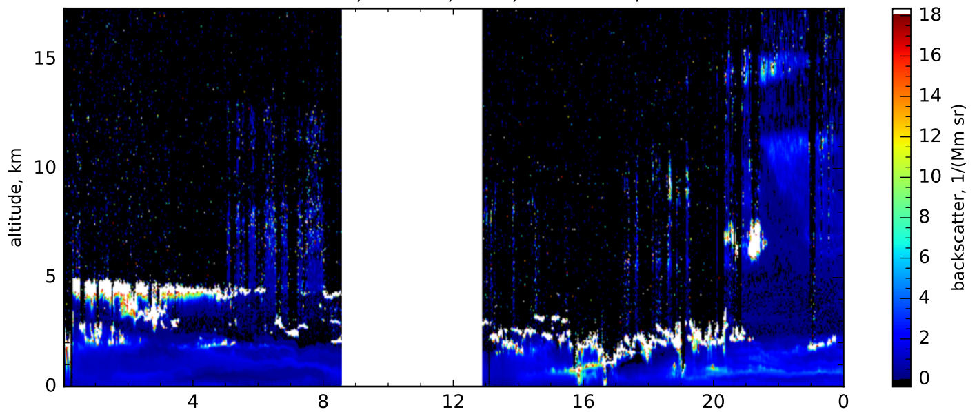
Particle backscatter, 532nm, near, res.: 120s, 60m-660m
