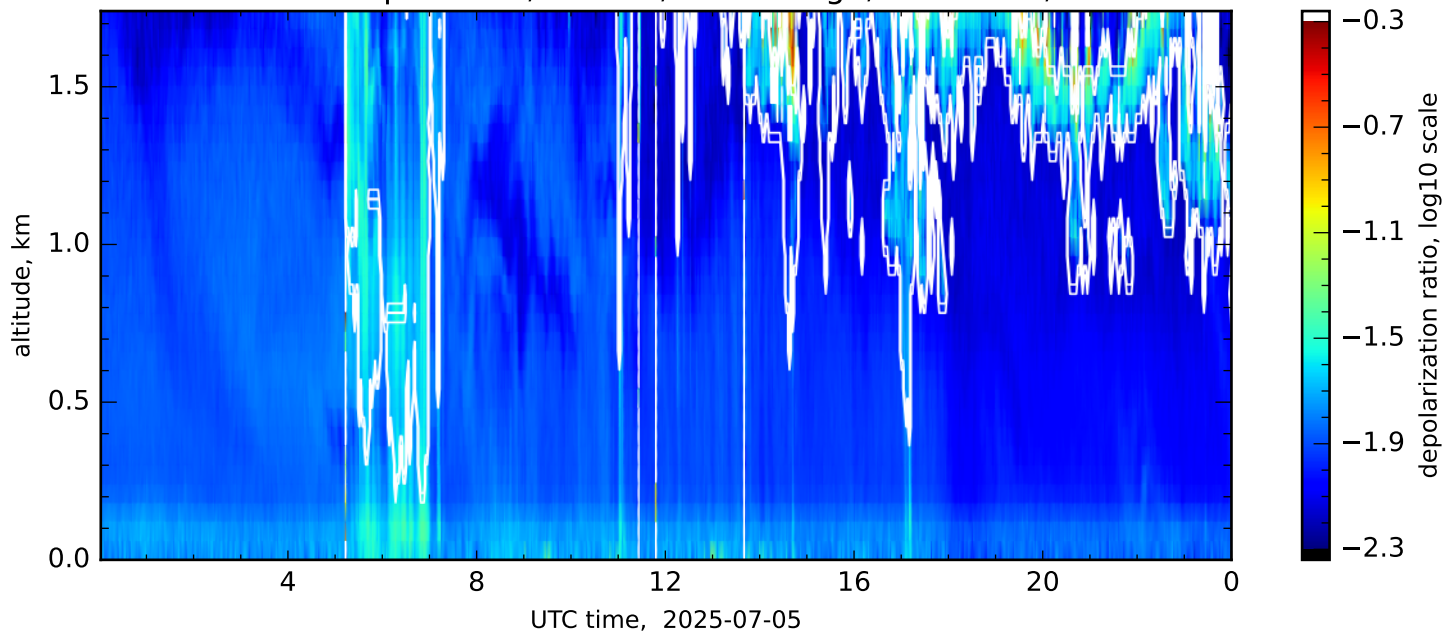
Volume linear depol. ratio, 532nm, close range, res.: 120s, 60m-60m
